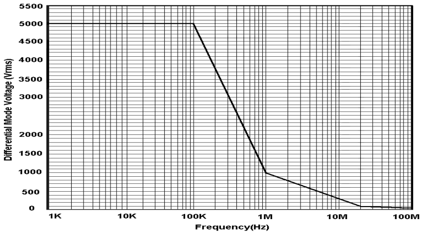
Derating Curve TT-SI 8010A, 8010B
