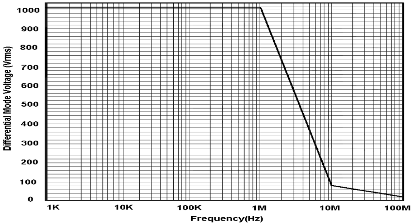
Derating Curve TT-SI 8050, 8051, 8052
